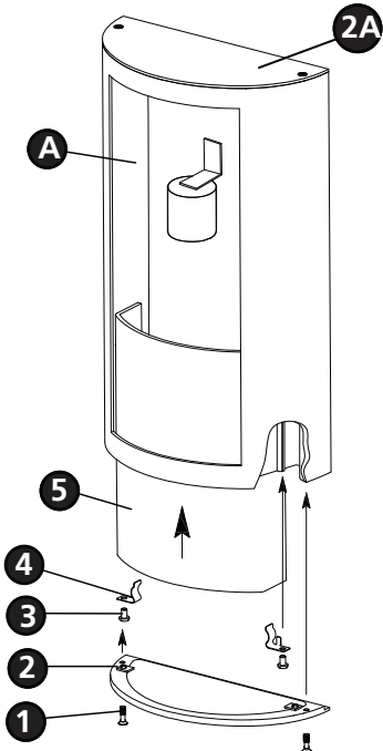
Drawing 3 - Detail Drawing
